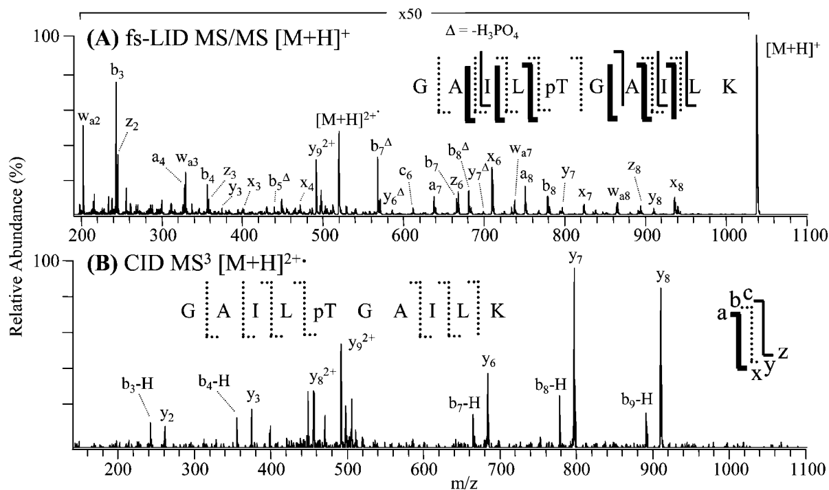
Figure 2. (A) fs-LID MS/MS (200 msec irradiation) of the [M + H]^+ precursor ion of GAILpTGAILK. (B) CID MS 3 of the [M + H]^{2+} photoionization product from panel A.
